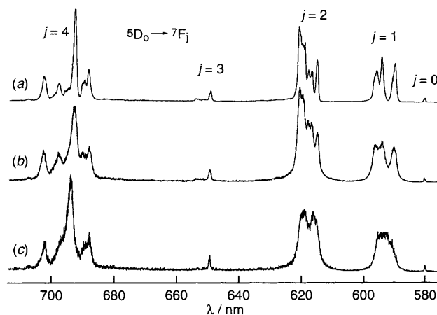
Fig. 2 Luminescence spectra of [EuZn(L 2 ) 3 ][ClO 4 ] 5 in the solid state at (a) 10 K, (b) 295 K and (c) in acetonitrile solution (295 K, 10 -3 mol dm -3 ), λ exc = 395 nm. Vertical scale: arbitrary units.
